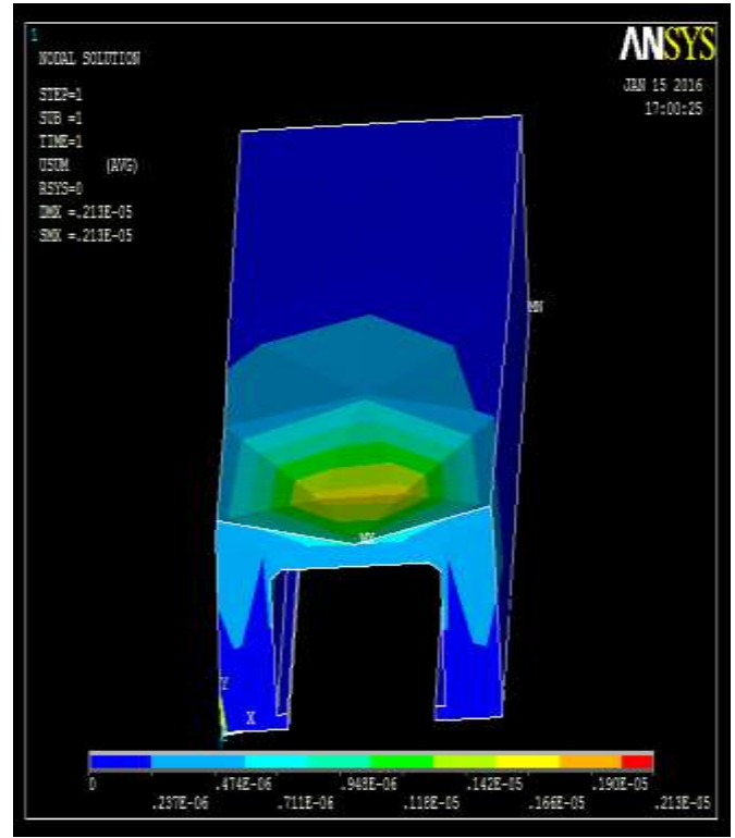
Figure 3 Displacement of bridge when load at 569 node
