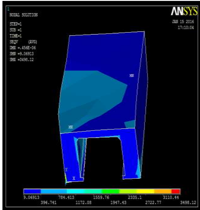
Figure 8 stress of bridge when load at node 209
