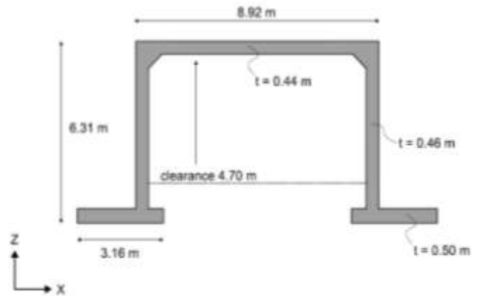
Figure 1 Bridge Structure Drawing
