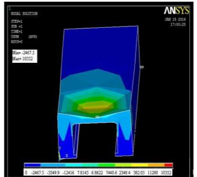
Figure 4 Stress of bridge when load at node 569
