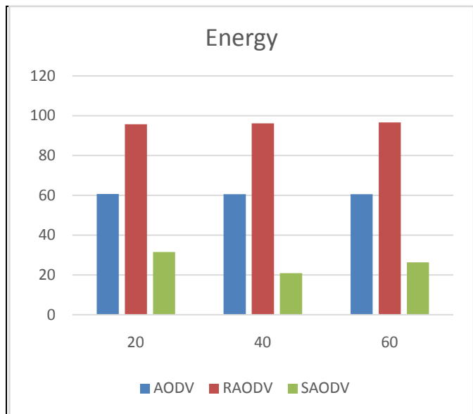
Figure. 3: Residual Energy under AODV, RAODV and SAODV
