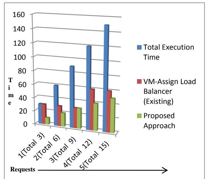
Figure 3: Graph to show time complexity comparison
