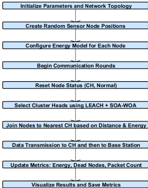
Figure 1. System Architecture
