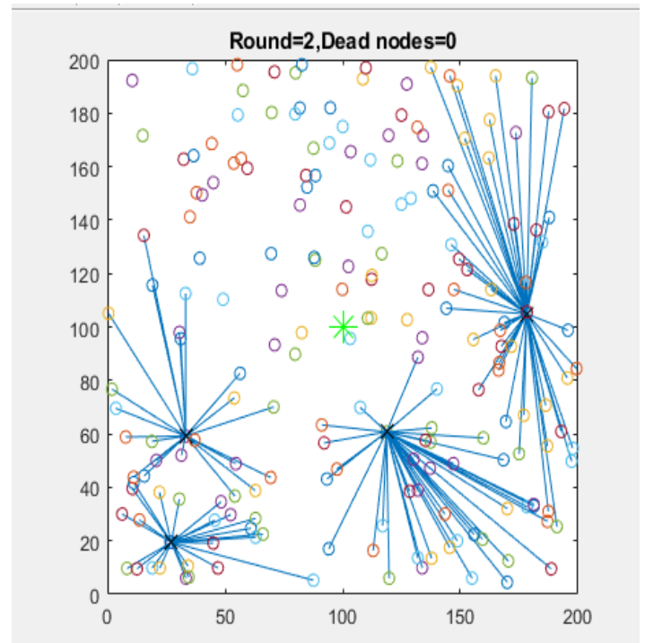
Figure 2. system initialization
