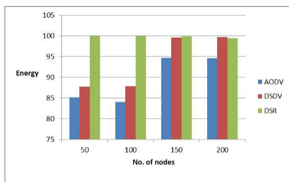
Fig 4: Residual Energy
