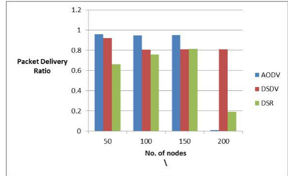
Fig 1: Packet Delivery Ratio
