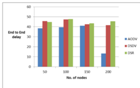
Fig 3: End to End Delay
